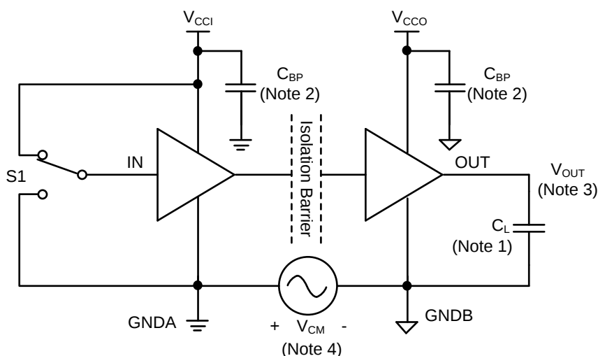
Figure 10-3. Default Output Delay Time Test Circuit and Voltage Waveforms
