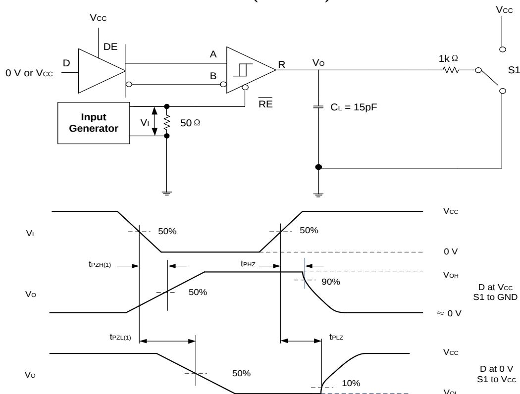
Figure 7-7. Measurement of Receiver Enable/Disable Times With Driver Enabled
