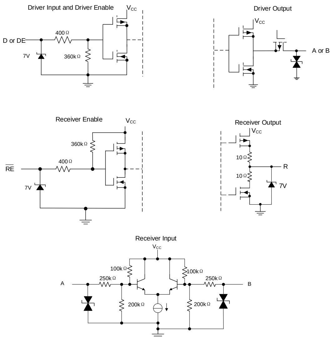
Figure 13. Equivalent Input and Output Schematic Diagrams
