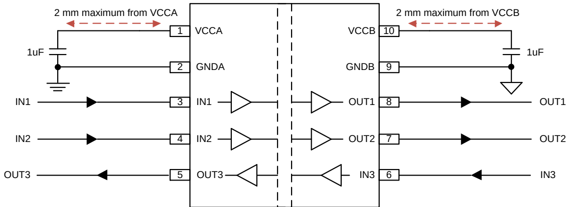
Figure 12-1. UMISO7331U Typical Application
