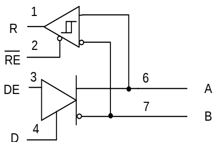
UM3783 Simplified Schematic
