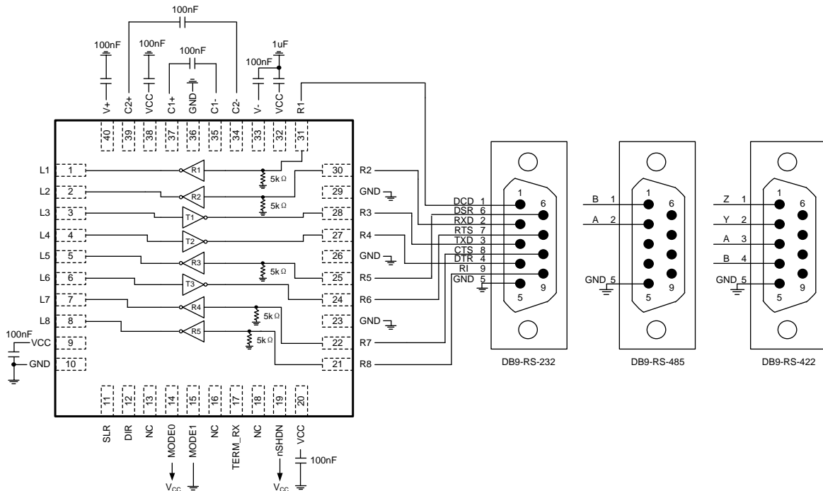
Figure 11-3. UM3035B Application on a shared DB9 connector
