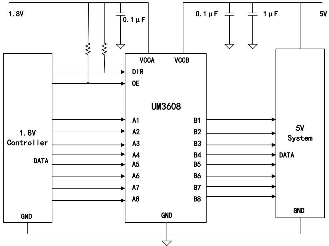
Typical Application Circuit
