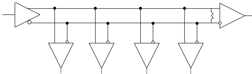
Figure 10-4. Multidrop or Distributed Simplex with Single Termination
