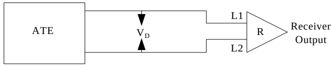
Figure 6. Receiver Propagation Delay Test Circuit
