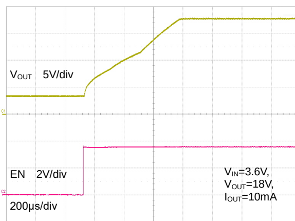
Start-up Behavior
