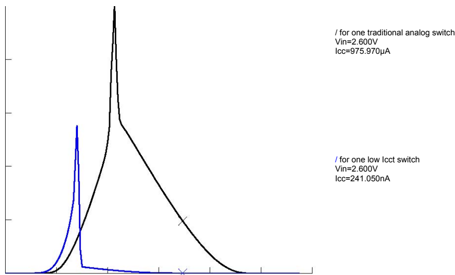
Figure 2. Icc vs. VIN for Low-Icct Switches vs. Traditional Analog Switches
