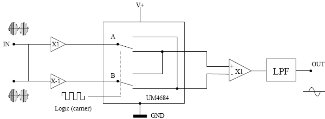
Fig 2: UM4684 as demodulator
