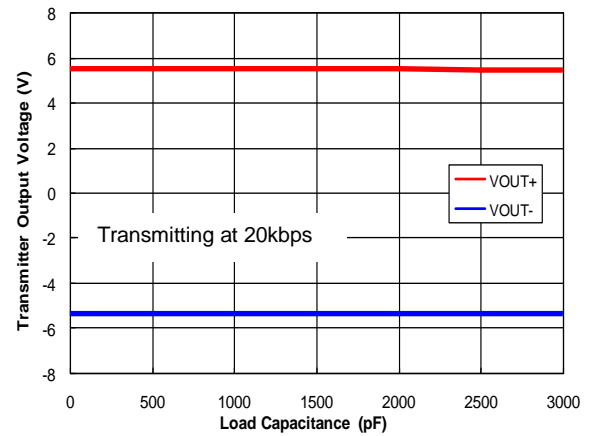
Transmitter Output Voltage vs. Load Capacitance
