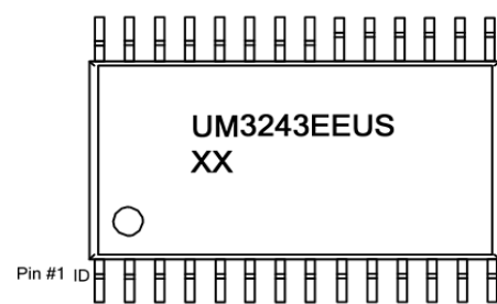
XX: Week Code UM3243EEUS TSSOP28
